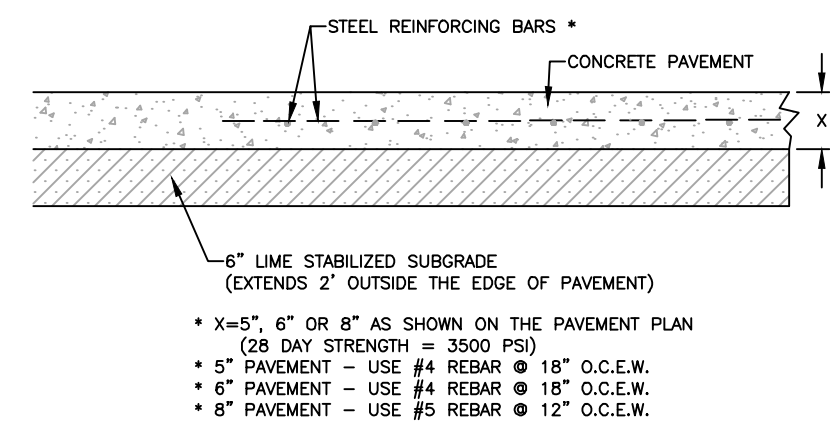
CONCRETE PAVING SECTION DETAIL - TYPICAL N.T.S.
