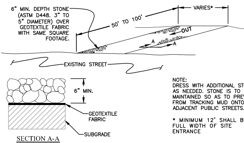
CONSTRUCTION EXIT SILT CONTROL DETAIL N.T.S.
