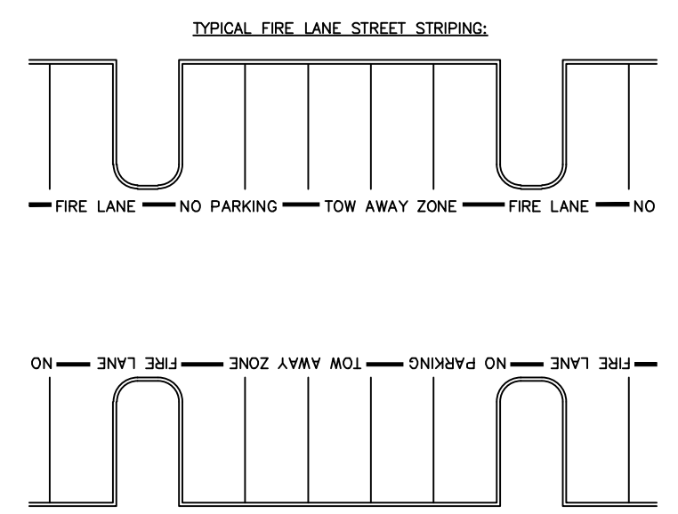
FIRE LANE STRIPING AND SIGNAGE DETAIL N.T.S.
