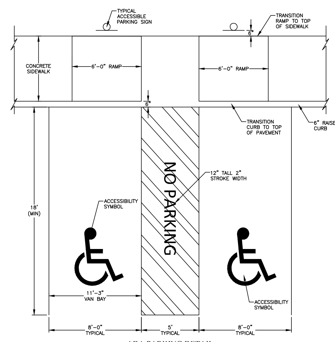
ADA PARKING DETAIL N.T.S.
