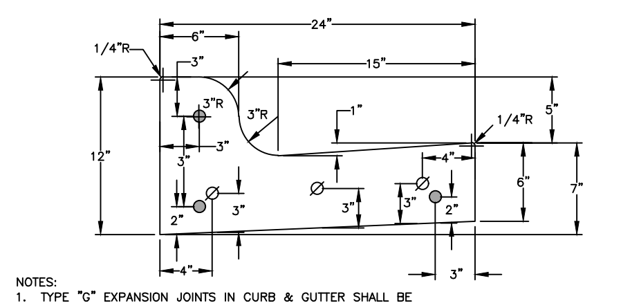
COMBINED CURB AND GUTTER SECTION DETAIL - TYPICAL N.T.S.
